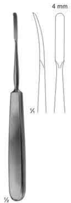
16-122 JOSEPH 170 mm
